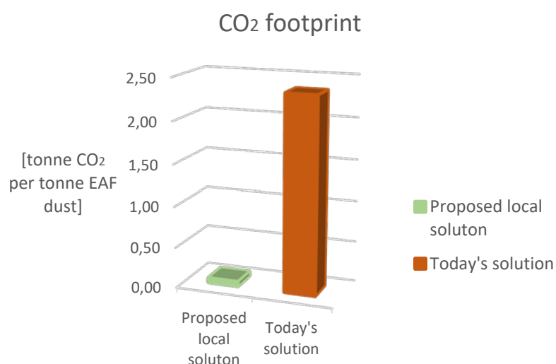
Figure 3: Comparison of total estimated CO 2 emissions from today's solution versus the proposed local solution (from stored EAF dust to processed zinc metal) (see Appendix A11).
