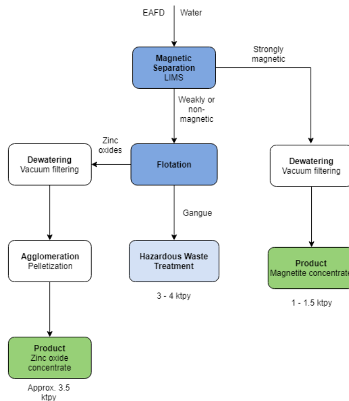
Figure 7: Preliminary EAFF circuit (also in Fig.5; repeated for convenience)
